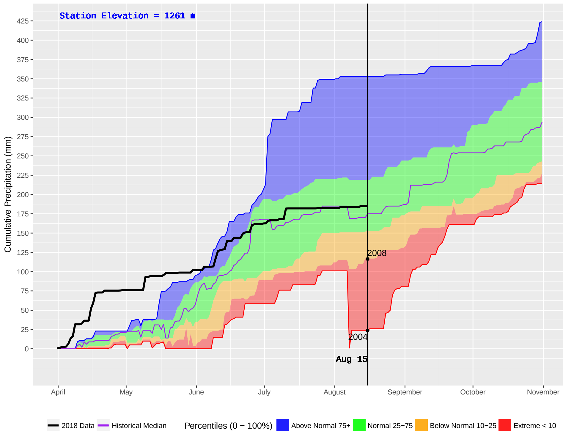
IDA BELL LAKE 3 (876) : Historical (2004–2016) and Current (2018) Daily Cumulative Precipitation
