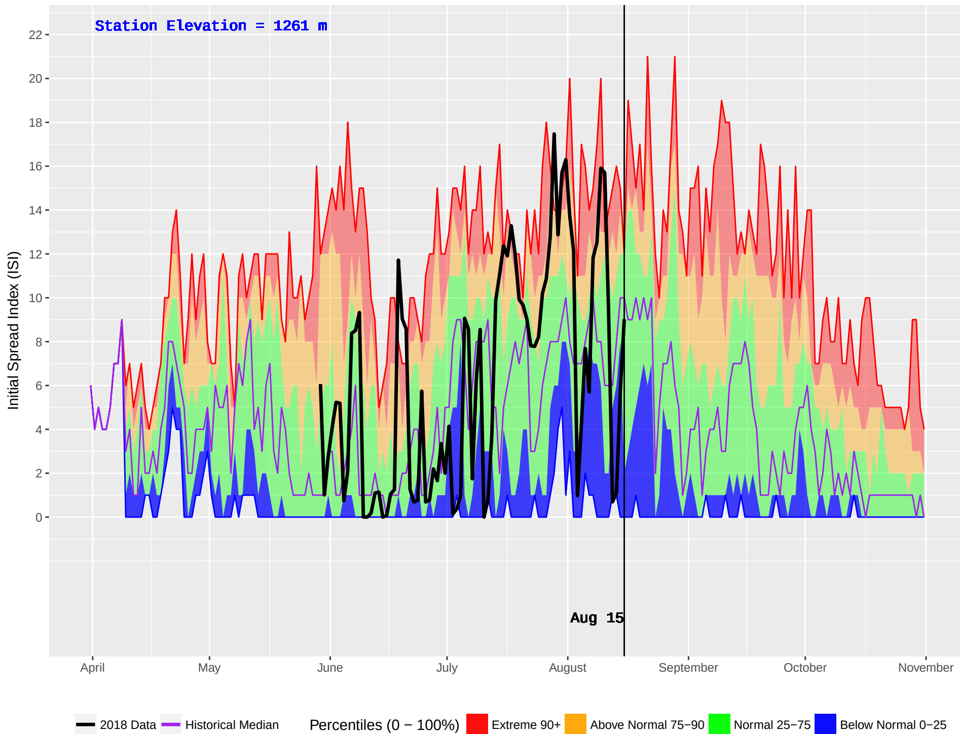
IDA BELL LAKE 3 (876) : Historical (2004–2016) and Current (2018) Daily Initial Spread Index (ISI)
