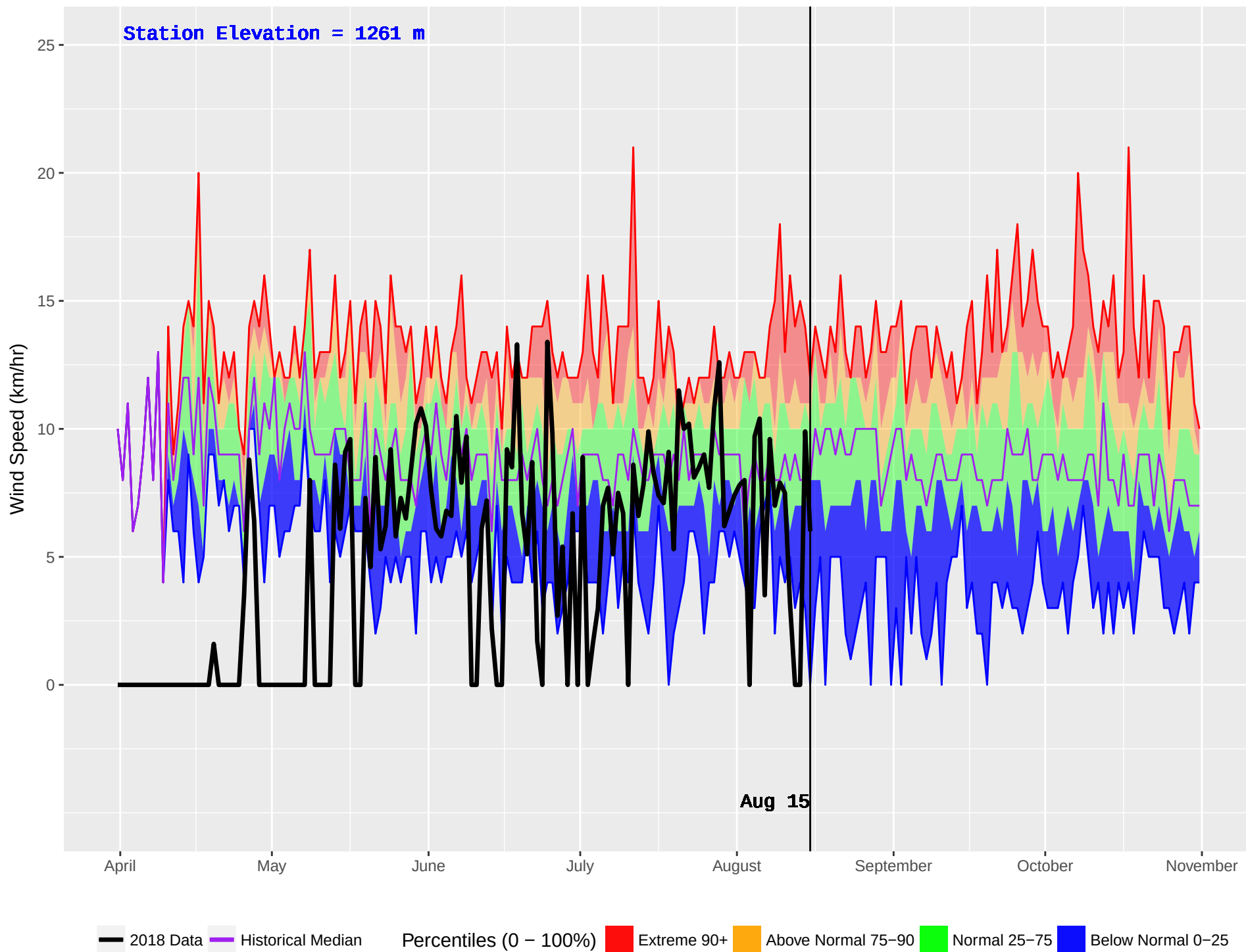
IDA BELL LAKE 3 (876) : Historical (2004–2016) and Current (2018) Daily Wind Speed
