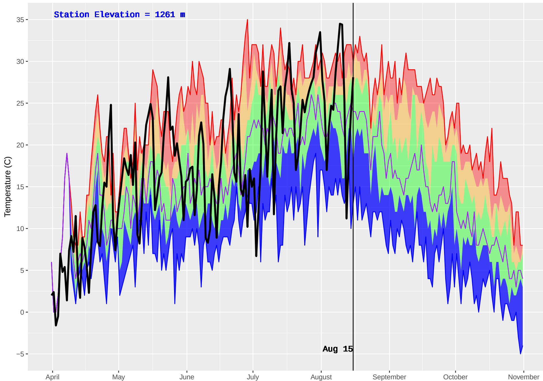
IDA BELL LAKE 3 (876) : Historical (2004–2016) and Current (2018) Daily Temperature
