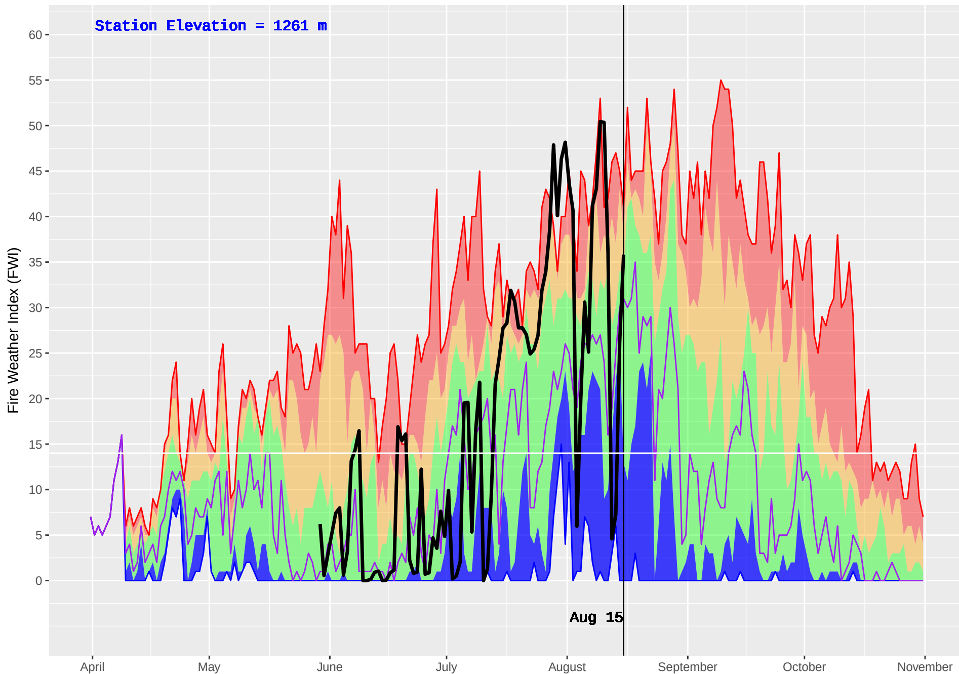
IDA BELL LAKE 3 (876) : Historical (2004–2016) and Current (2018) Daily Fire Weather Index (FWI)
