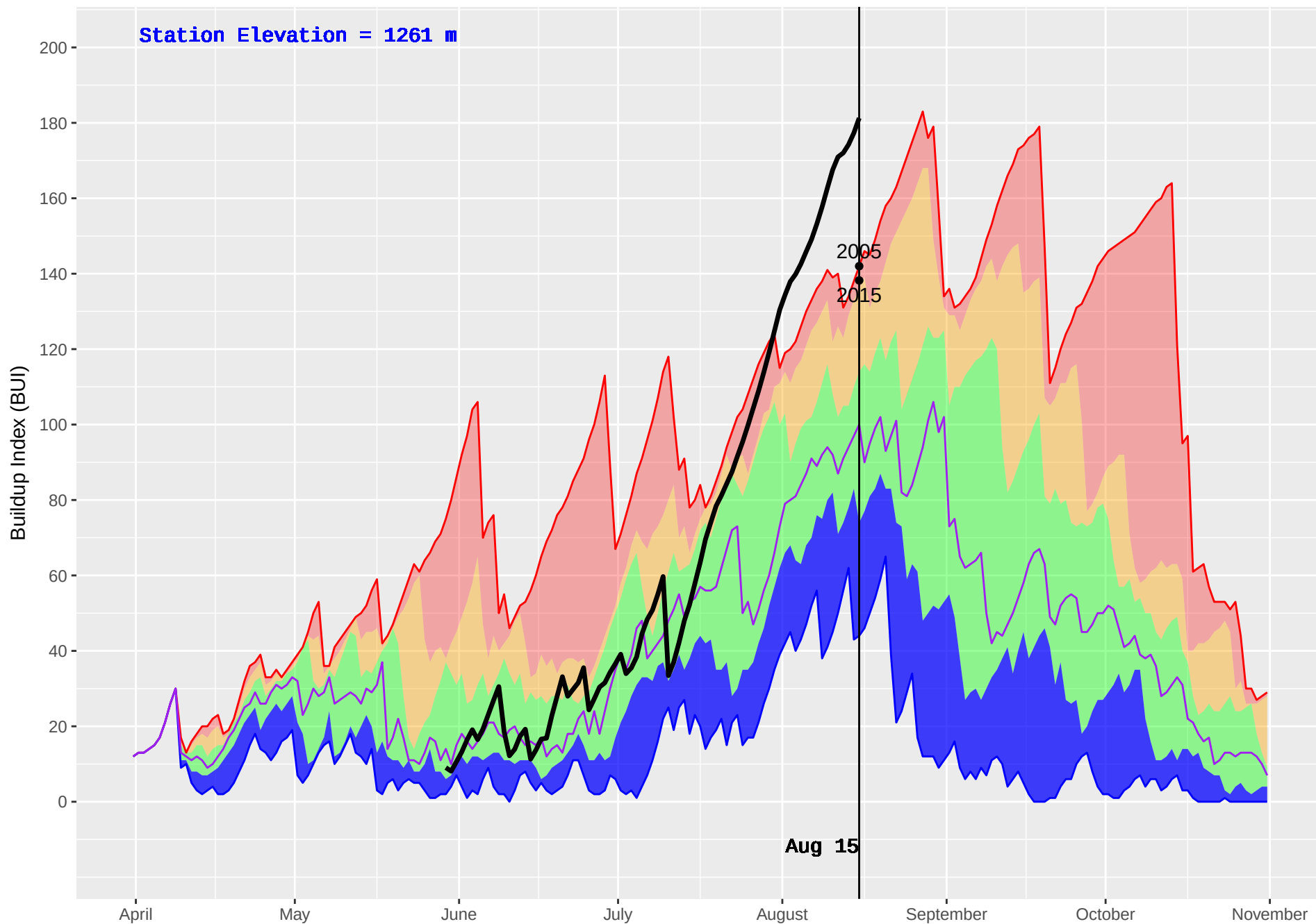
IDA BELL LAKE 3 (876) : Historical (2004–2016) and Current (2018) Daily Buildup Index (BUI)
