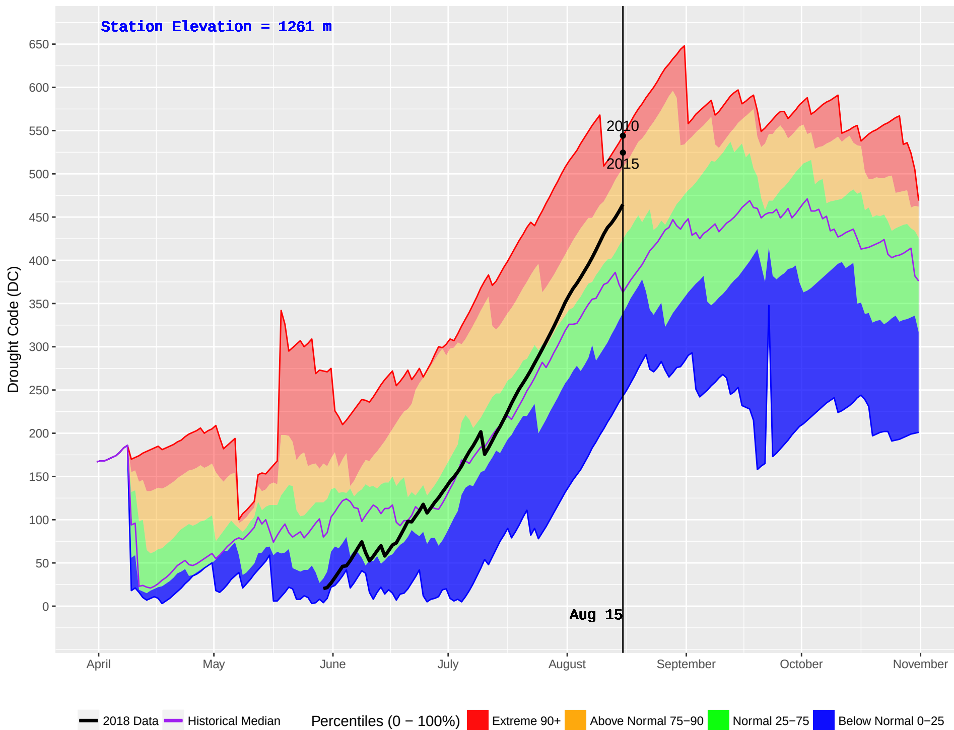
IDA BELL LAKE 3 (876) : Historical (2004–2016) and Current (2018) Daily Drought Code (DC)
